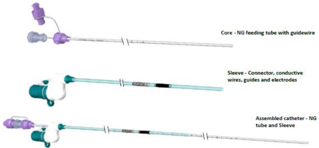
Figure 7: Phagenyx Catheter
